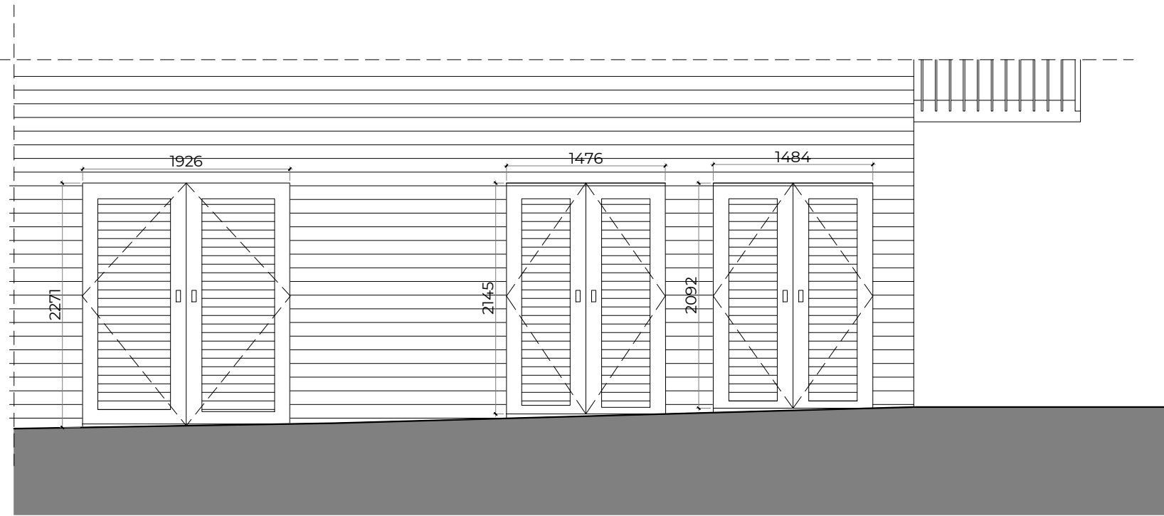
REFUSE & STORAGE FRONT ELEVATION
