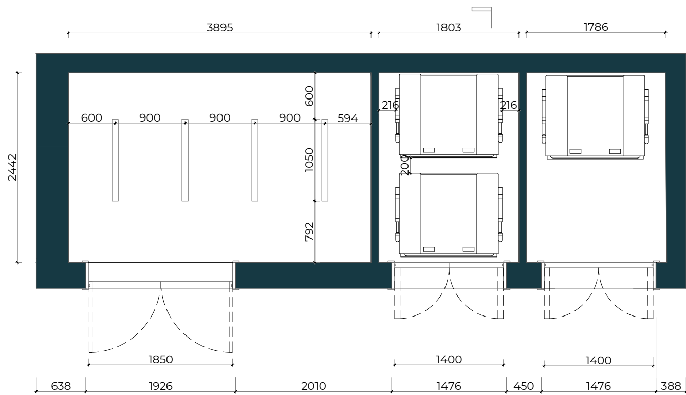
REFUSE & STORAGE FLOOR PLAN
