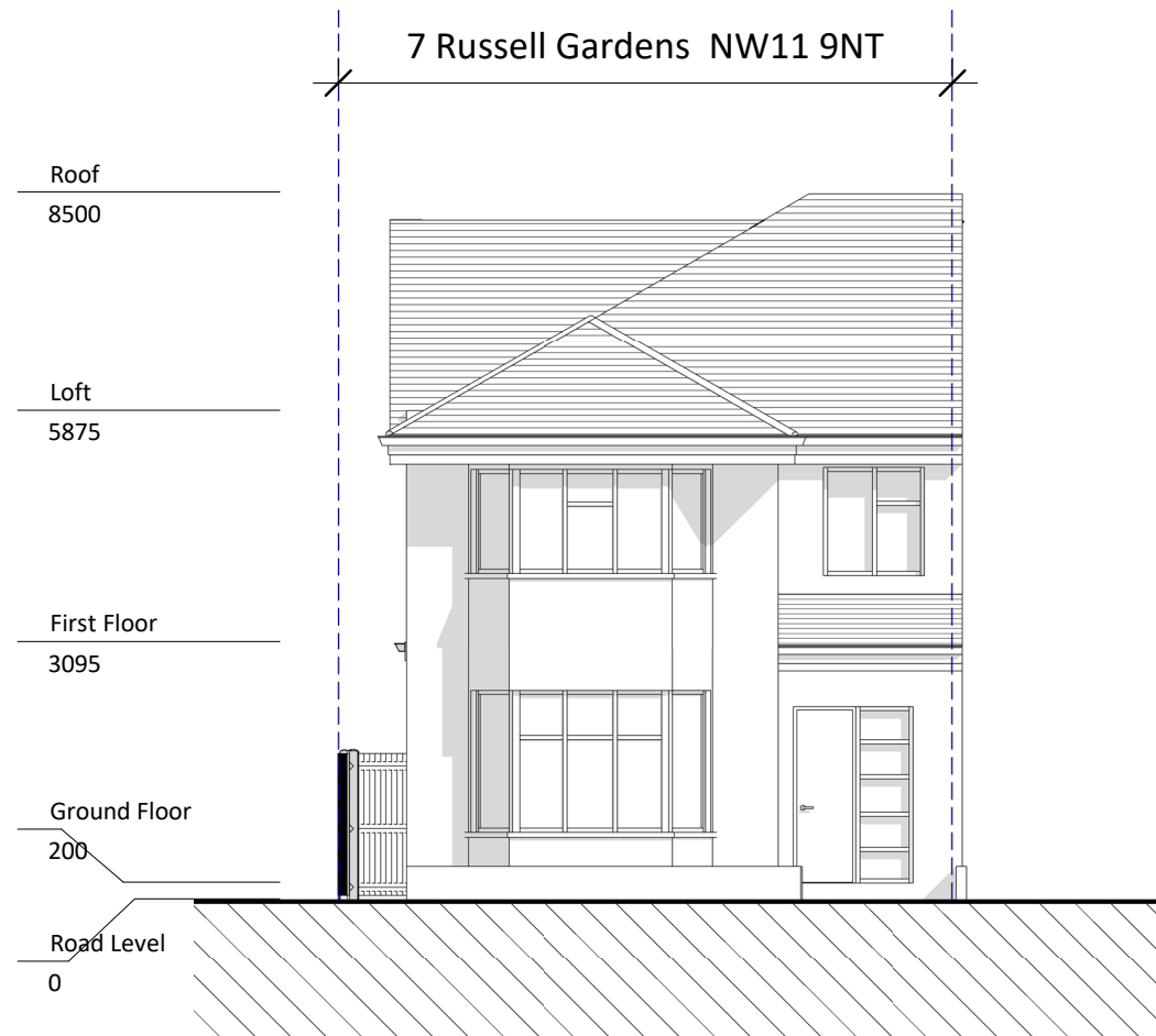
FRONT ELEVATION
