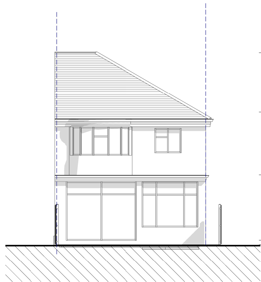
REAR ELEVATION
