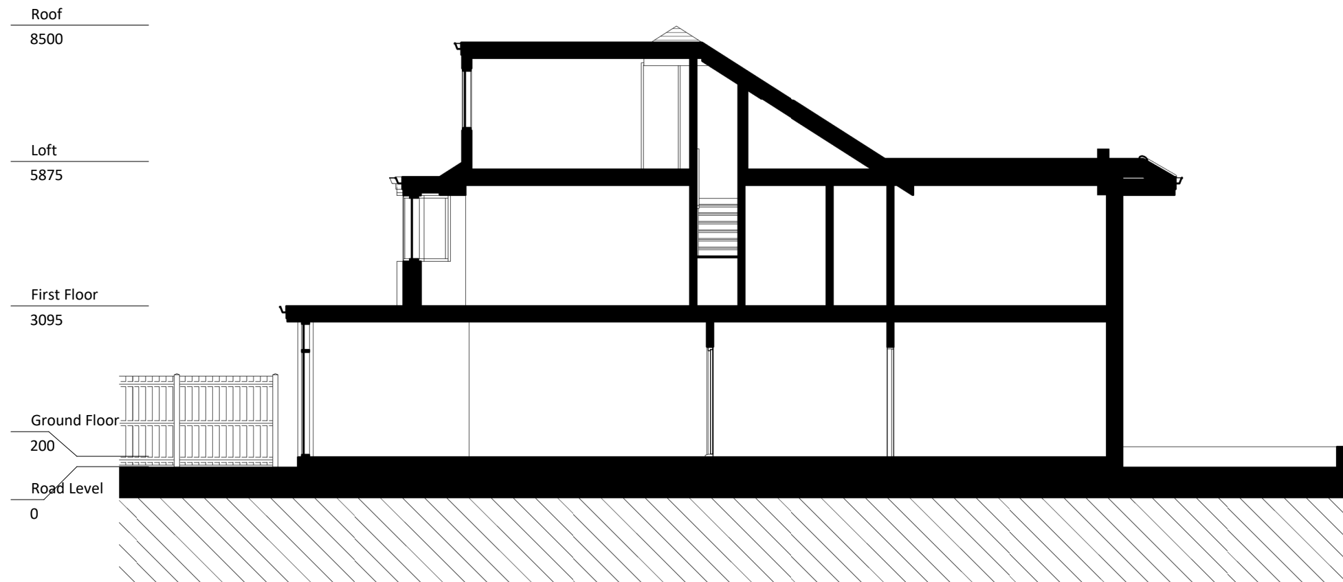
SECTION AA
