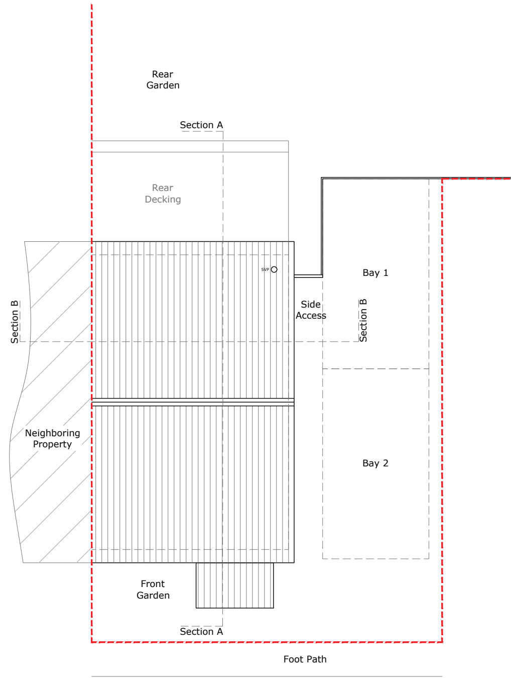
3 Existing Roof Plan 1:100
