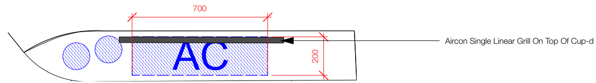
1 Plan 1:20 @ A3
