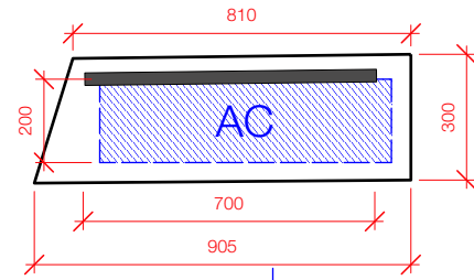
1 Left Side Unit Plan 1:20 @ A3
