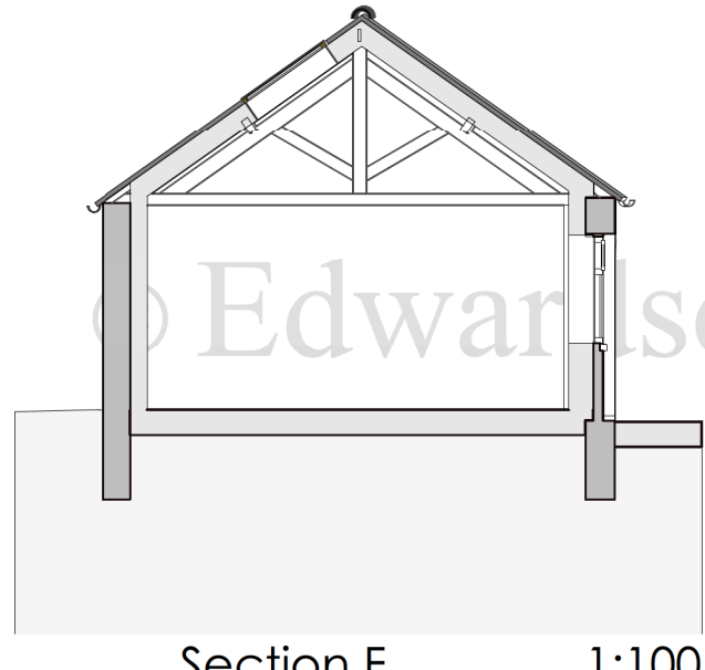
Section F 1:100
