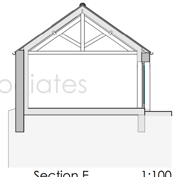
Section E 1:100
