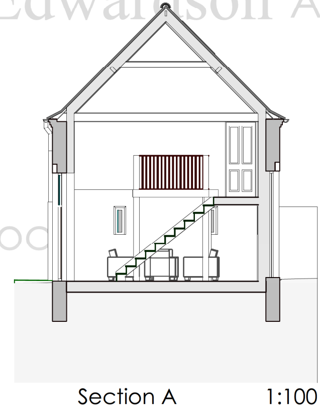
Section A 1:100
