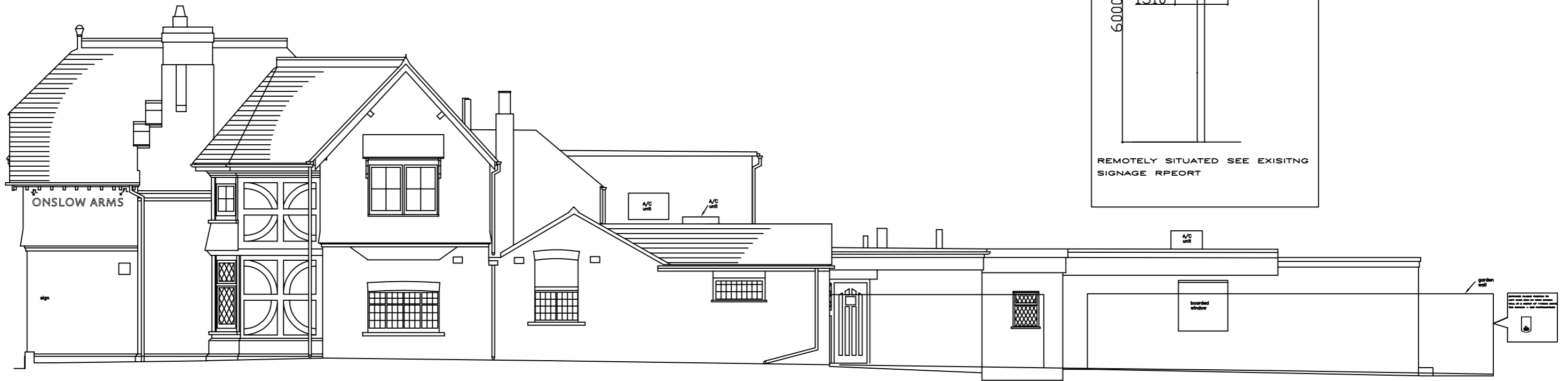
SIDE SOUTH FACING ELEVATION
