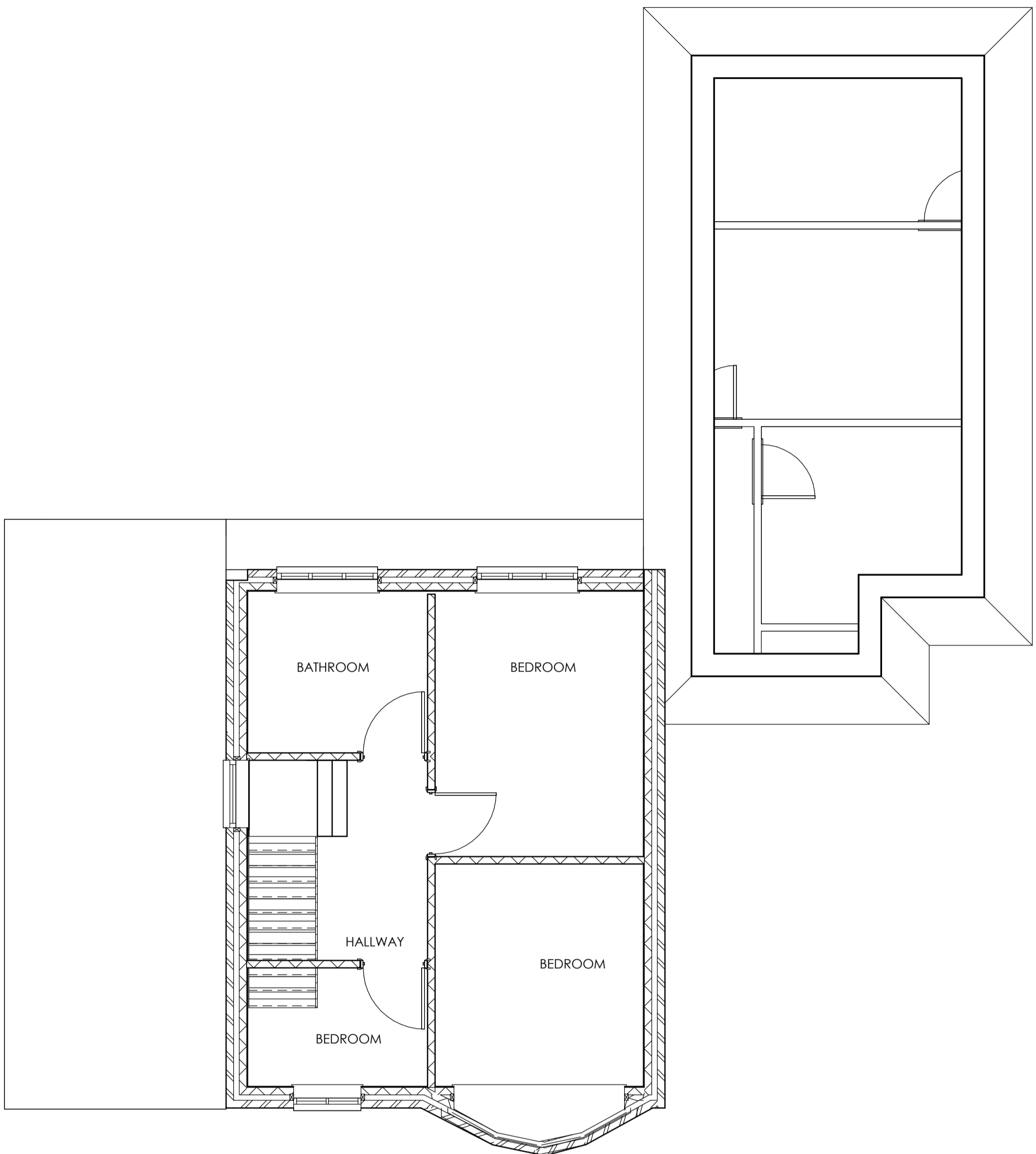
2 EXISTING FIRST FLOOR PLAN 1 : 50
