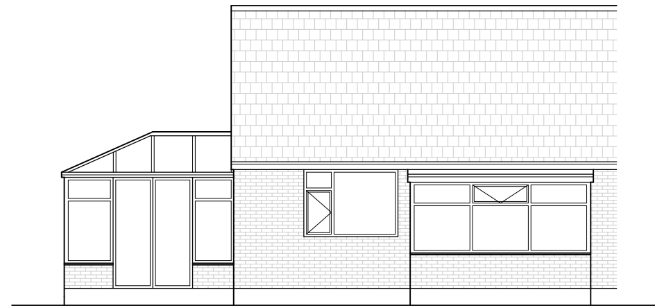
EXISTING REAR ELEVATION 1:100 @ A3
