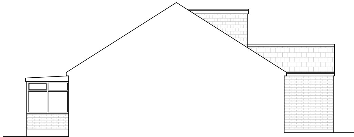
EXISTING SIDE ELEVATION 1:100 @ A3
