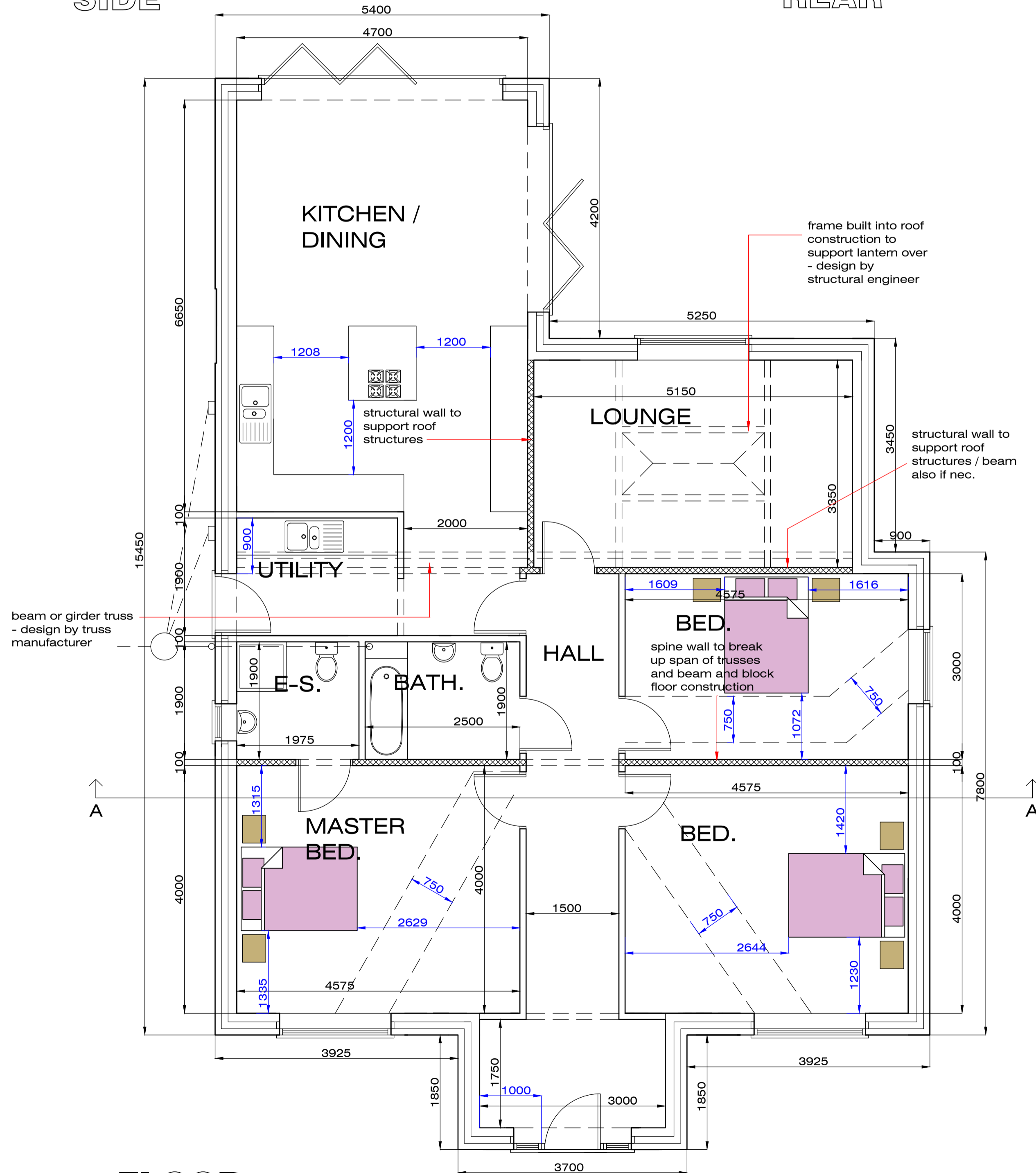
FLOOR PLAN
