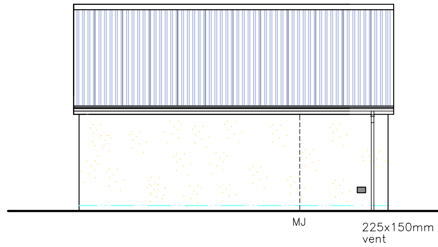
NORTH ELEVATION
