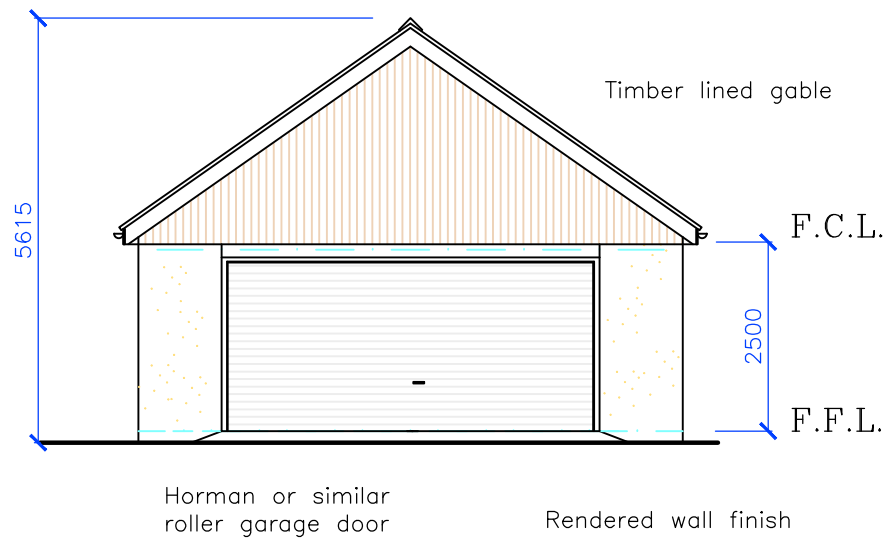
WEST ELEVATION
