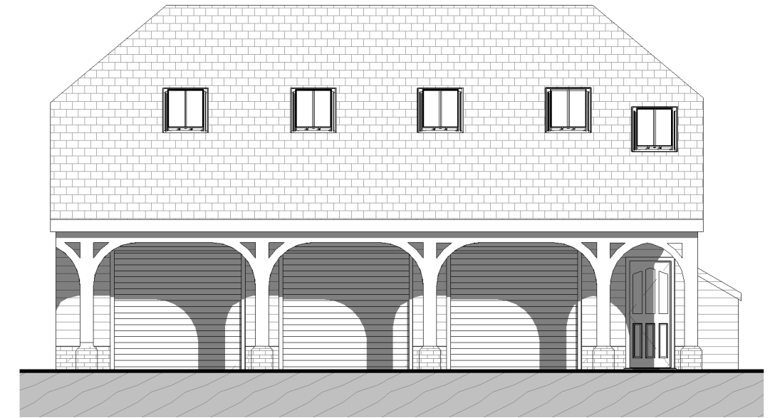
East Elevation 1 : 100
