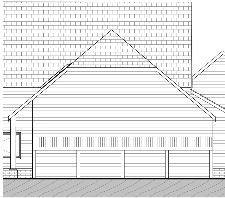
North Elevation 1 : 100
