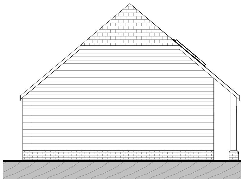
South Elevation 1 : 100
