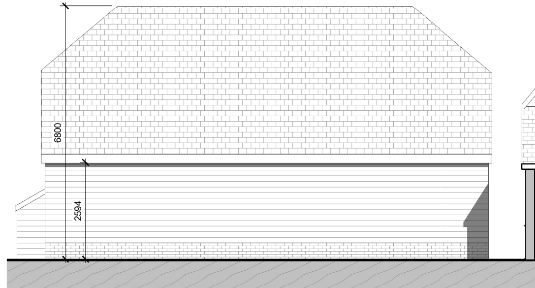
West Elevation 1 : 100
