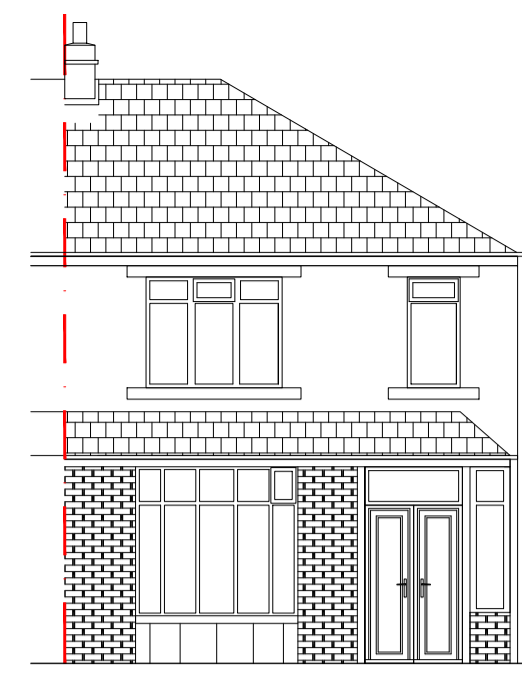
EXISTING FRONT ELEV. Scale 1:100@A1
