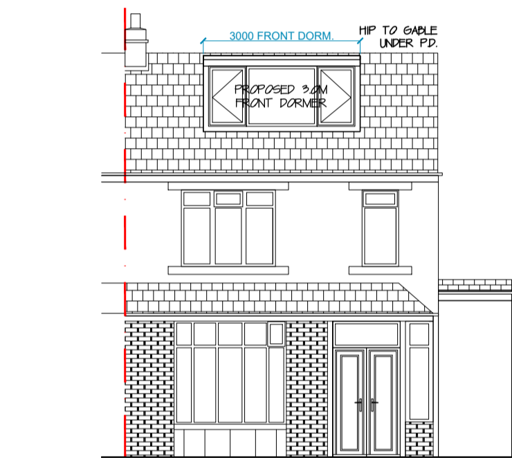
PROPOSED FRONT ELEV. Scale 1:100@A1
