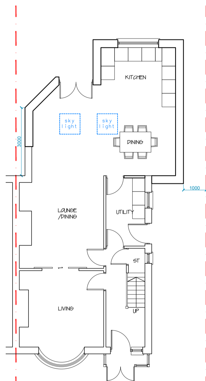
PROPOSED GROUND FLOOR Scale 1:100@A1
