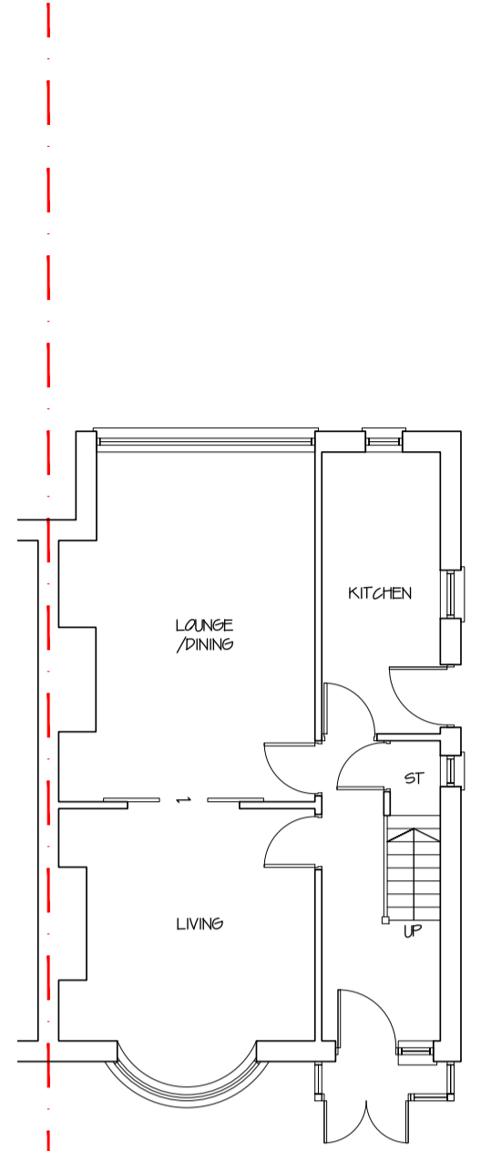
EXISTING GROUND FLOOR Scale 1:100@A1
