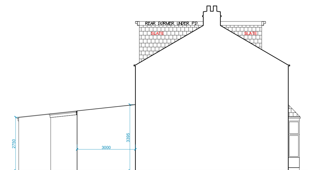
PROPOSED OTHER SIDE ELEV. Scale 1:100@A1
