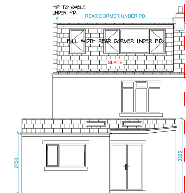
PROPOSED REAR ELEV. Scale 1:100@A1
