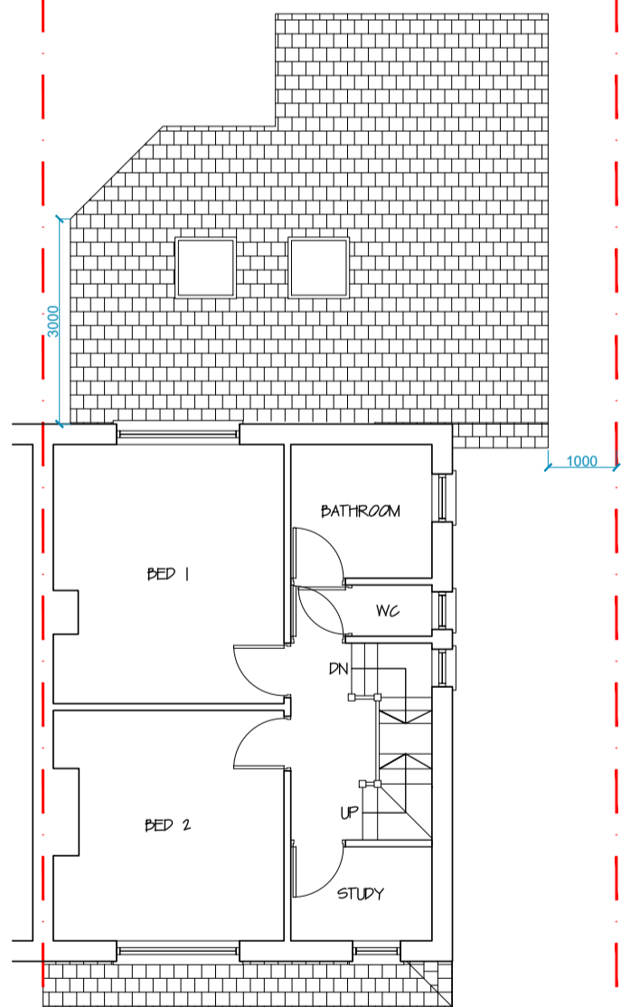
PROPOSED FIRST FLOOR Scale 1:100@A1
