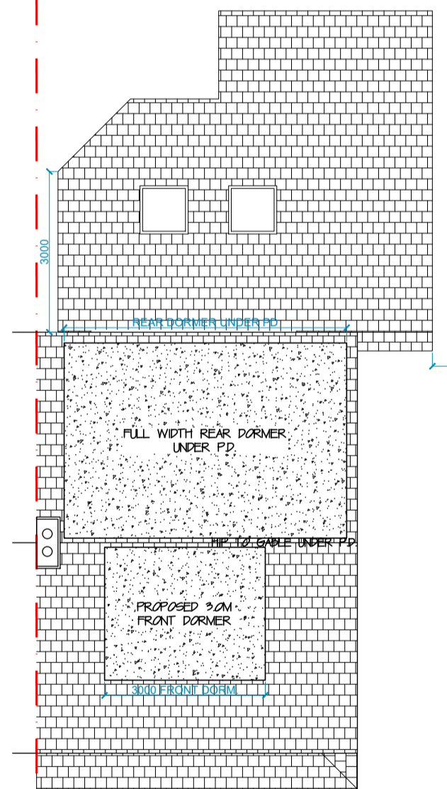
PROPOSED ROOF PLAN Scale 1:100@A1
