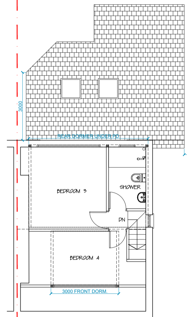
PROPOSED LOFT PLAN Scale 1:100@A1
