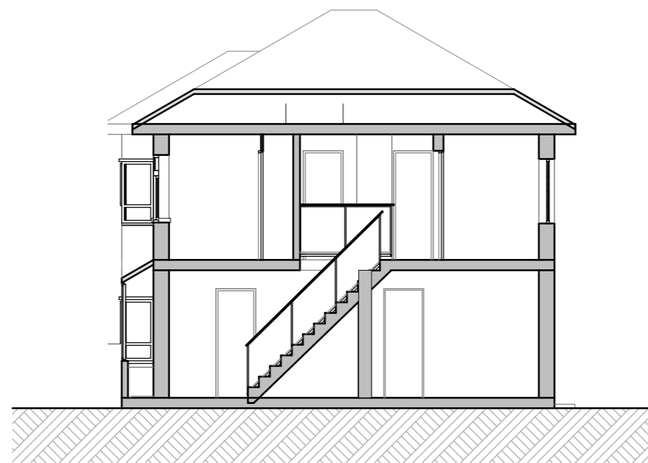
Building Section
