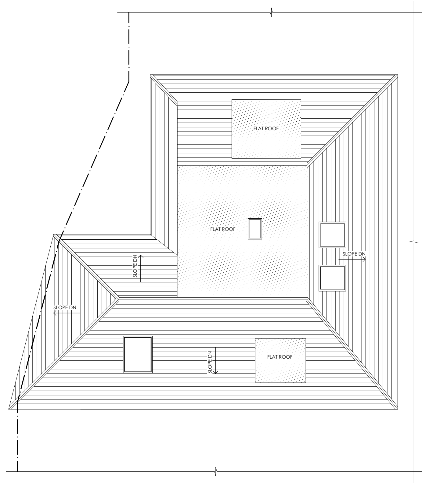
EXISTING ROOF (1:100 @ A3)
