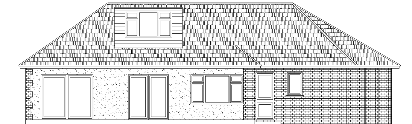
REAR ELEVATION (1:100 @ A3)
