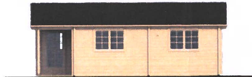
ARDEE CABIN GABLE FRONT ENTRANCE + DOWNHILL SIDE ELEVATIONS 1:100
