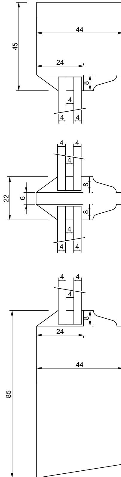
Selden, Ground Floor Flat, The Old Vicarage. Gibraltar Hill, Lincoln Windows A, B & C Drawing showing cross section of typical sash section, glazing bar section, bottom rail section and double glazed units with putty glazing. Scale 1:1
