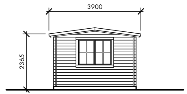
East Elevation
