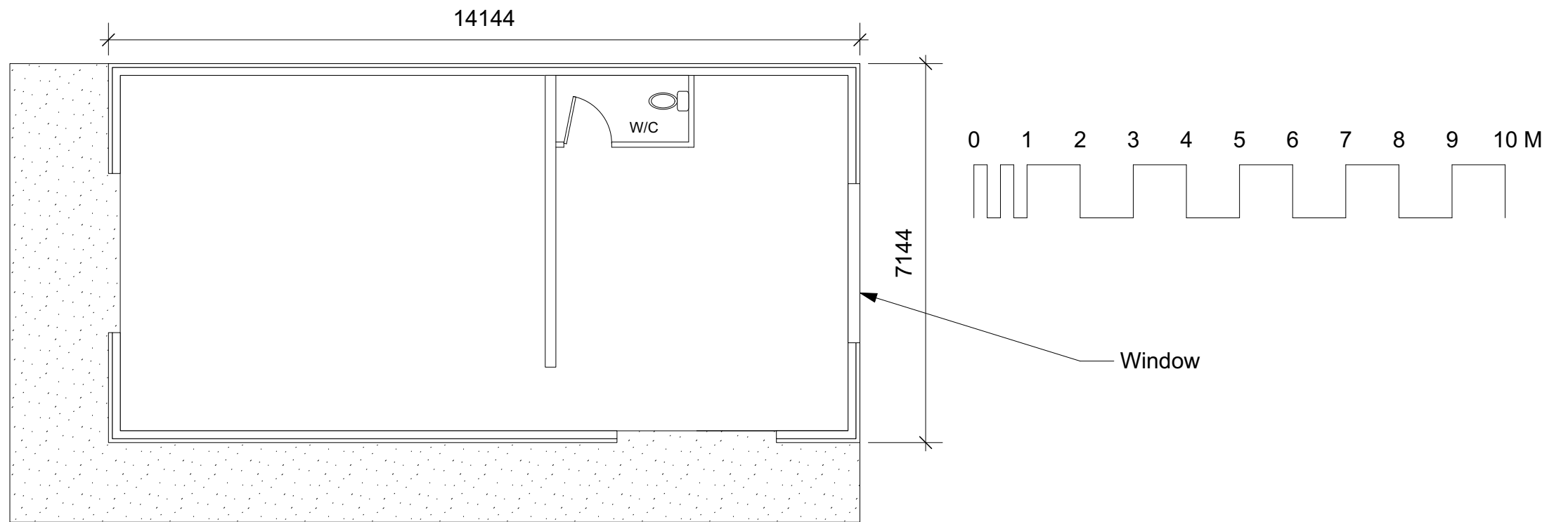
3 Floor & Roof Plan Scale: 1:100
