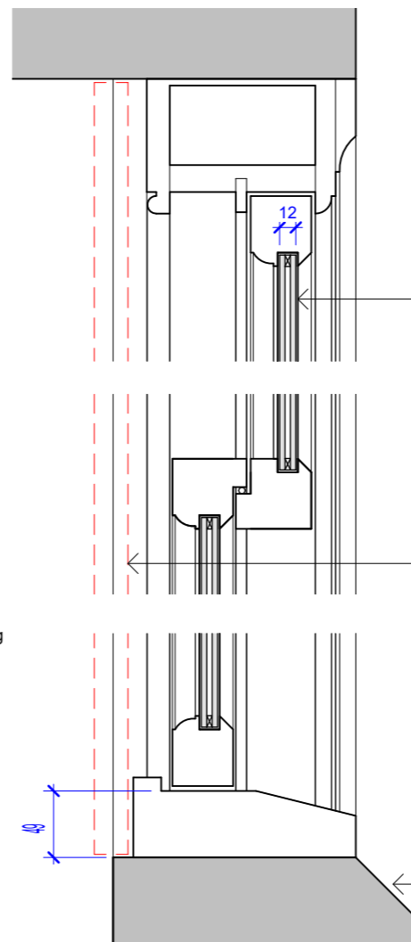
2 Sash Window Section 1 : 5
