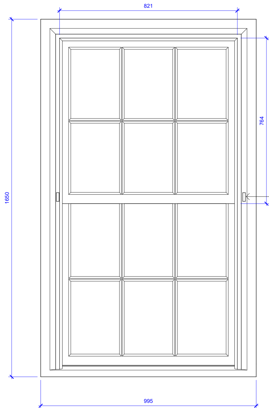
1 Sash Window Elevation 1 : 10
