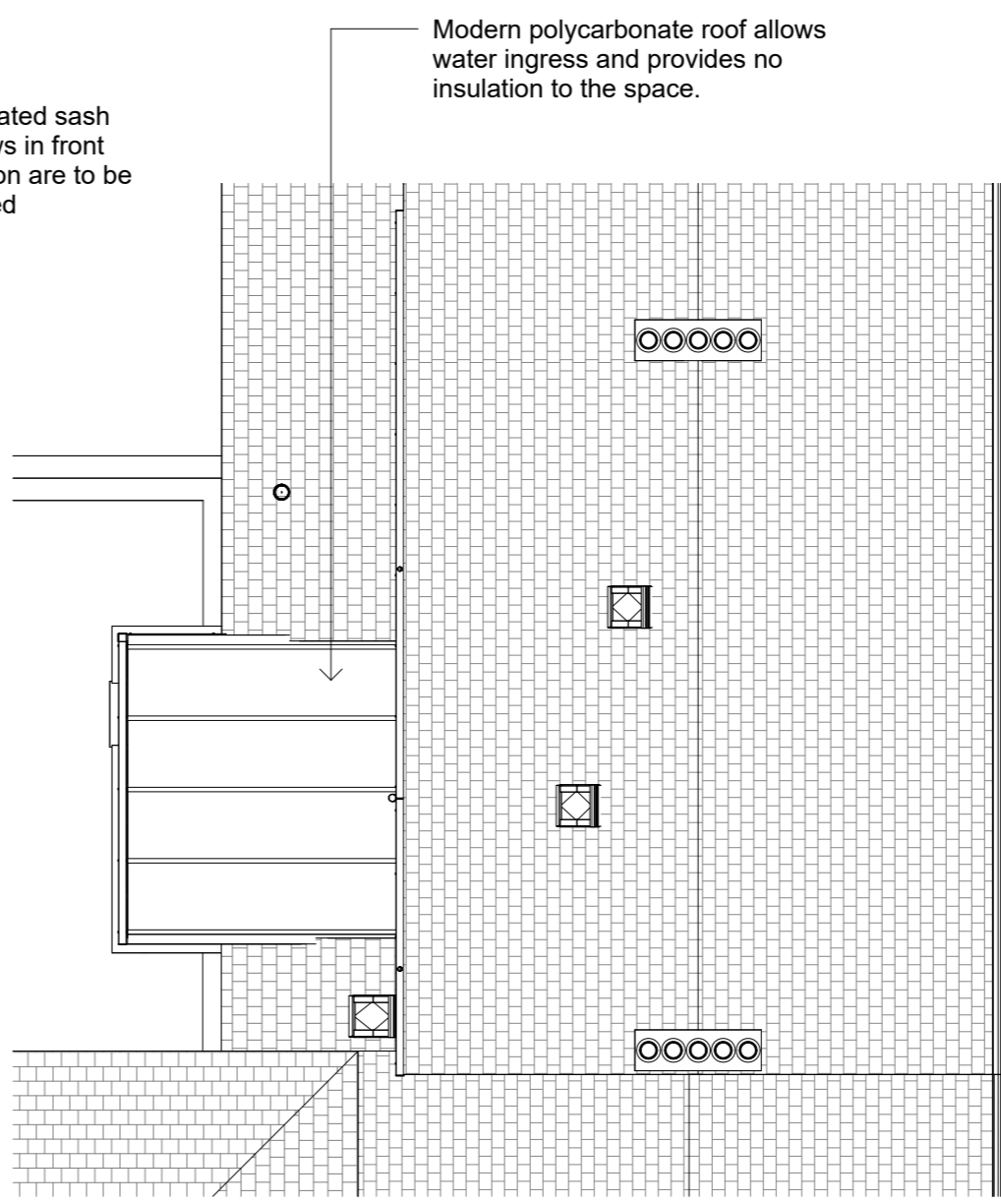
2 Existing Roof Plan 1 : 100
