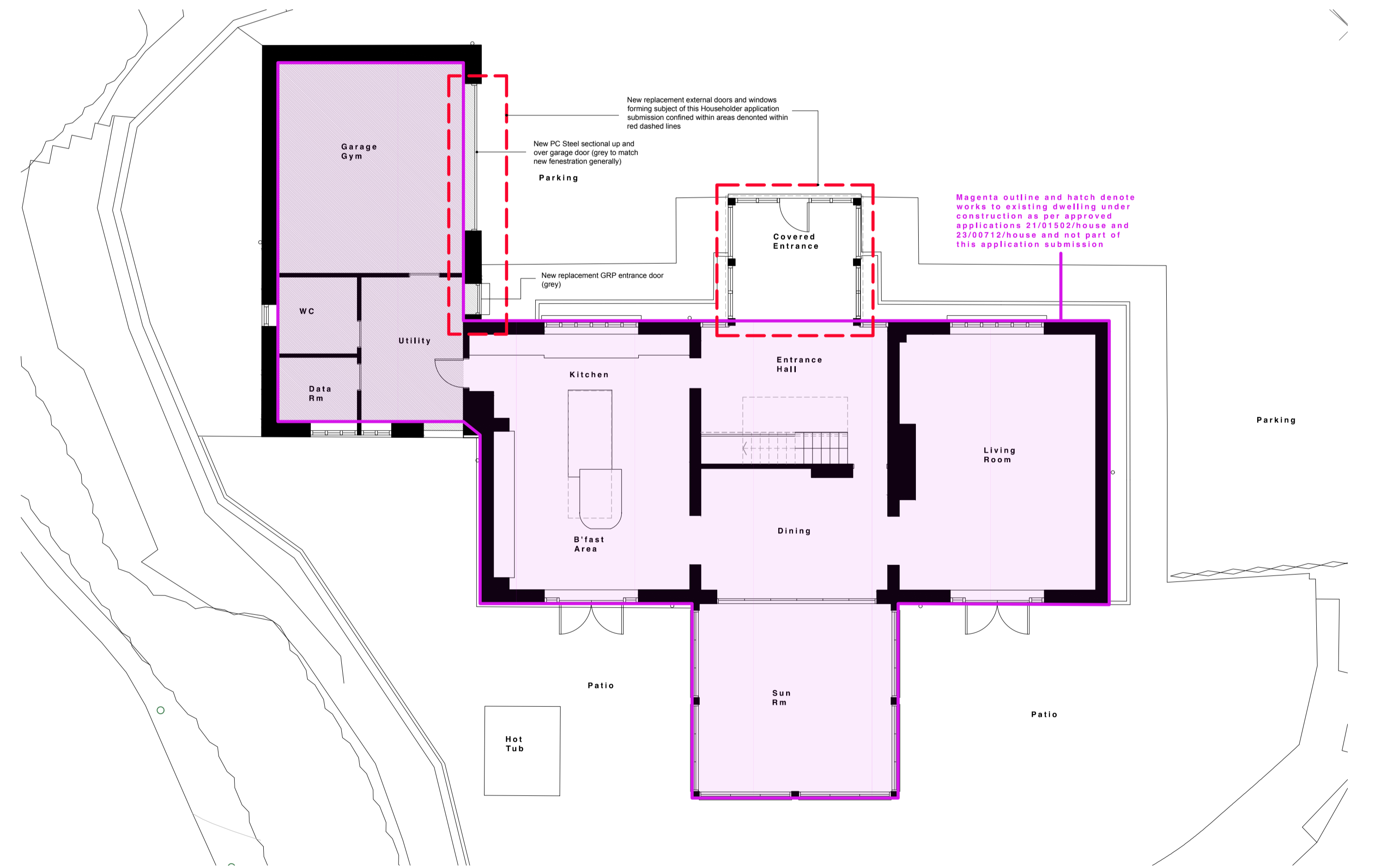
Ground Floor Plan [in context] - 1:100
