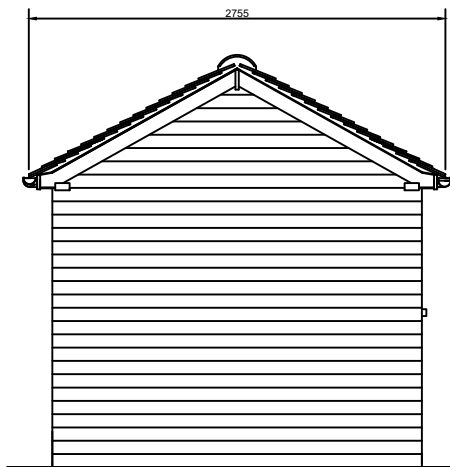
SIDE ELEVATION
