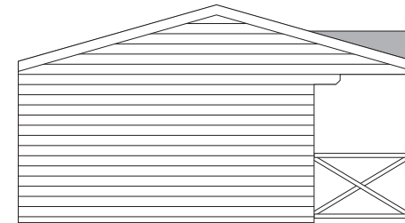
SIDE ELEVATION
