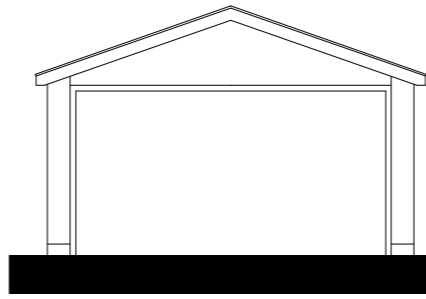
South Elevation | Existing
