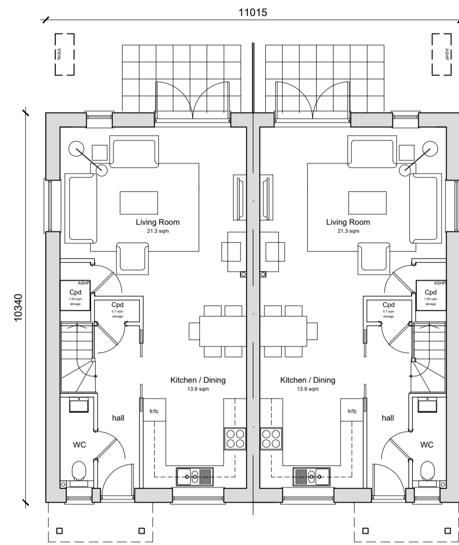
Ground Floor Plan Plot 10 3-Bedroom 5-Person House 95.1sqm / 1023 sqft GIA (to finishes) Min. 2.5sqm storage where shown to NDS requirements
