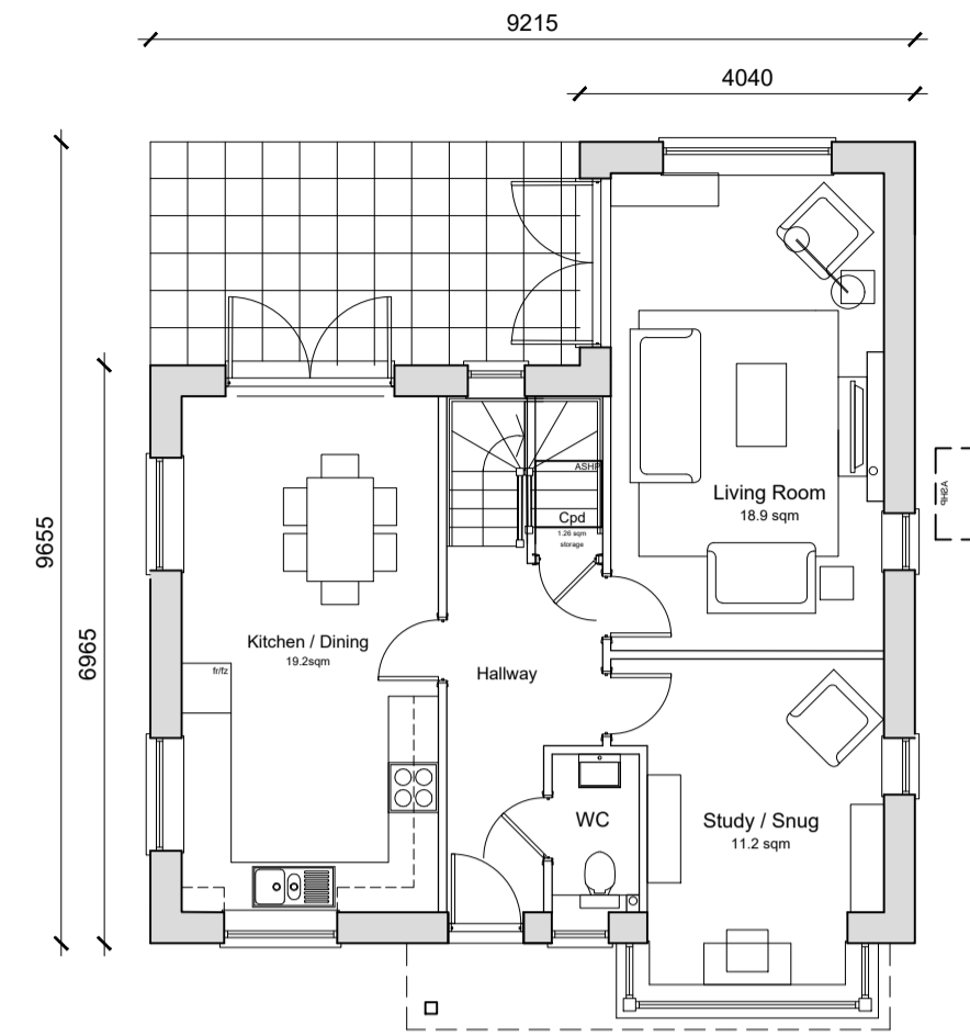
Ground Floor Plan Plot 2 3-Bedroom 5-Person House 124.9 sqm / 1345 sqft GIA (to finishes) Min. 2.5sqm storage where shown to NDSS requirements
