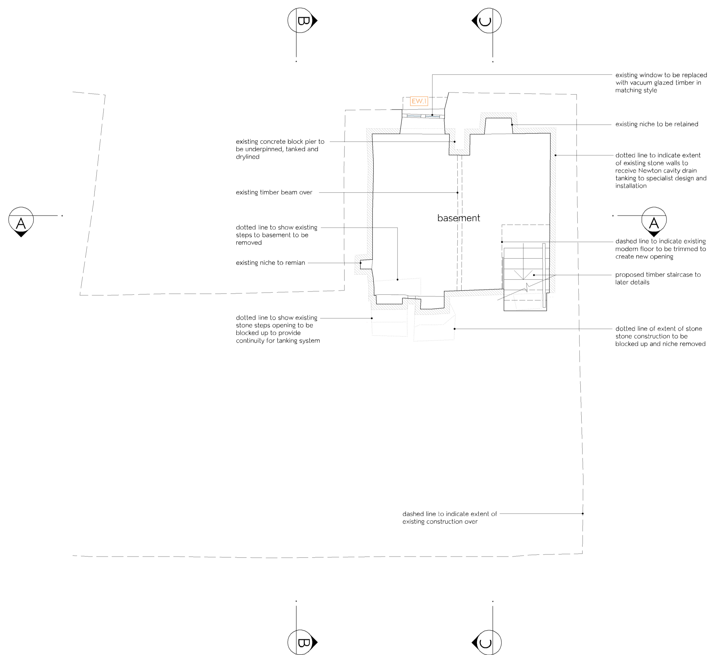
BASEMENT PLAN
