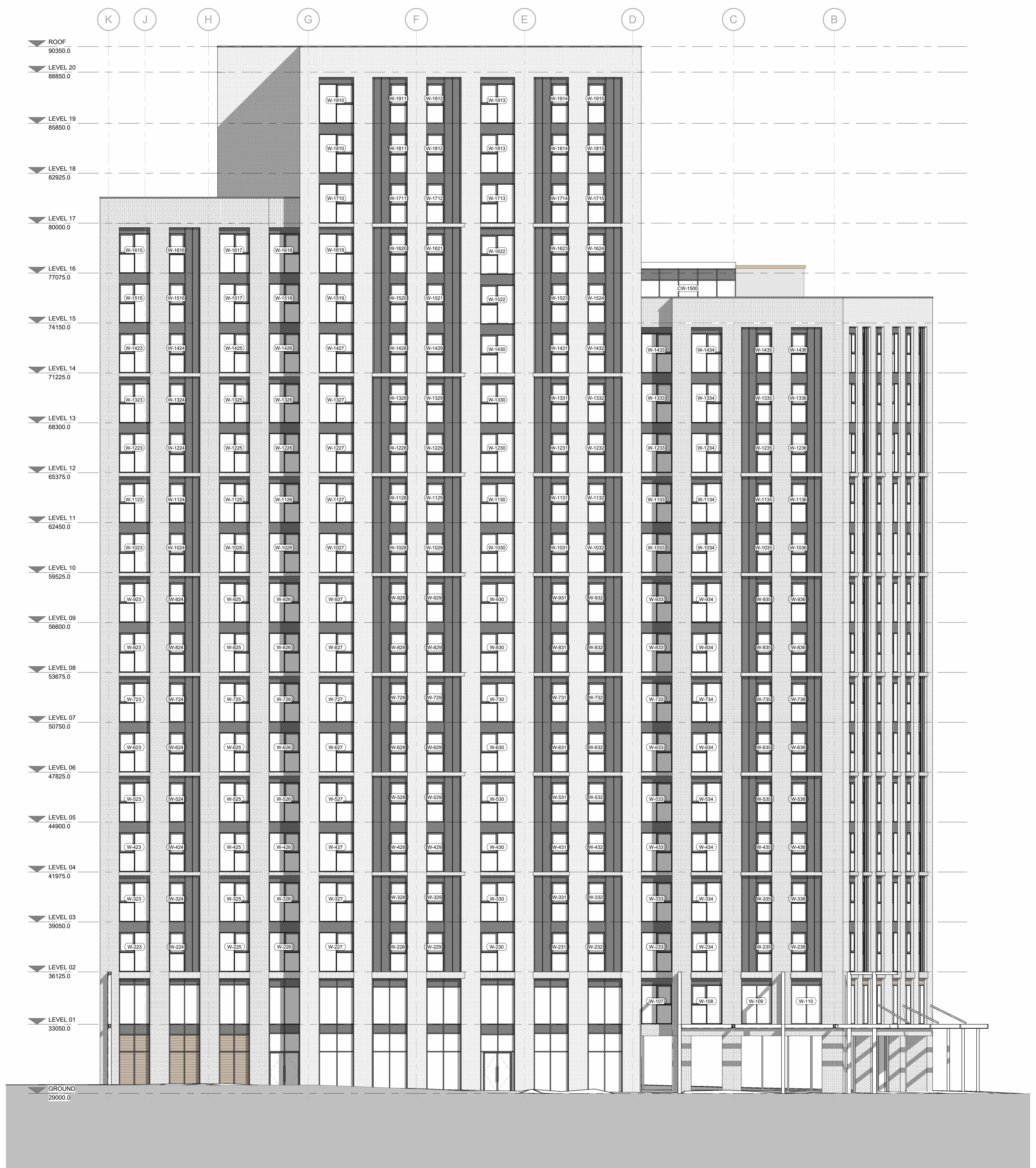
North Elevation
