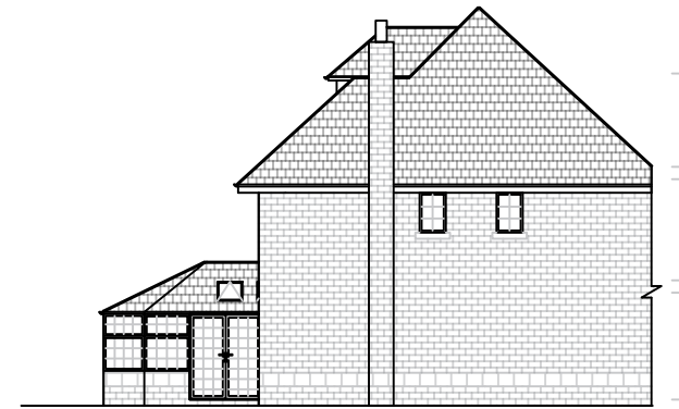
EXISTING SIDE ELEVATION SOUTH FACING
