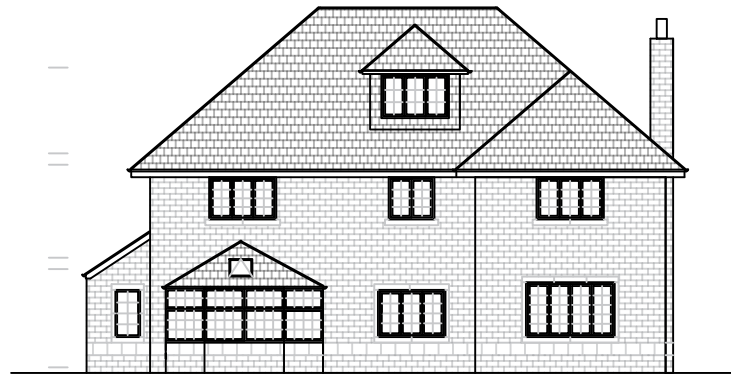
EXISTING REAR ELEVATION WEST FACING
