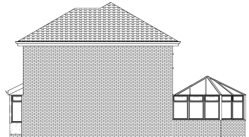
3 Side Elevation 1 : 100
