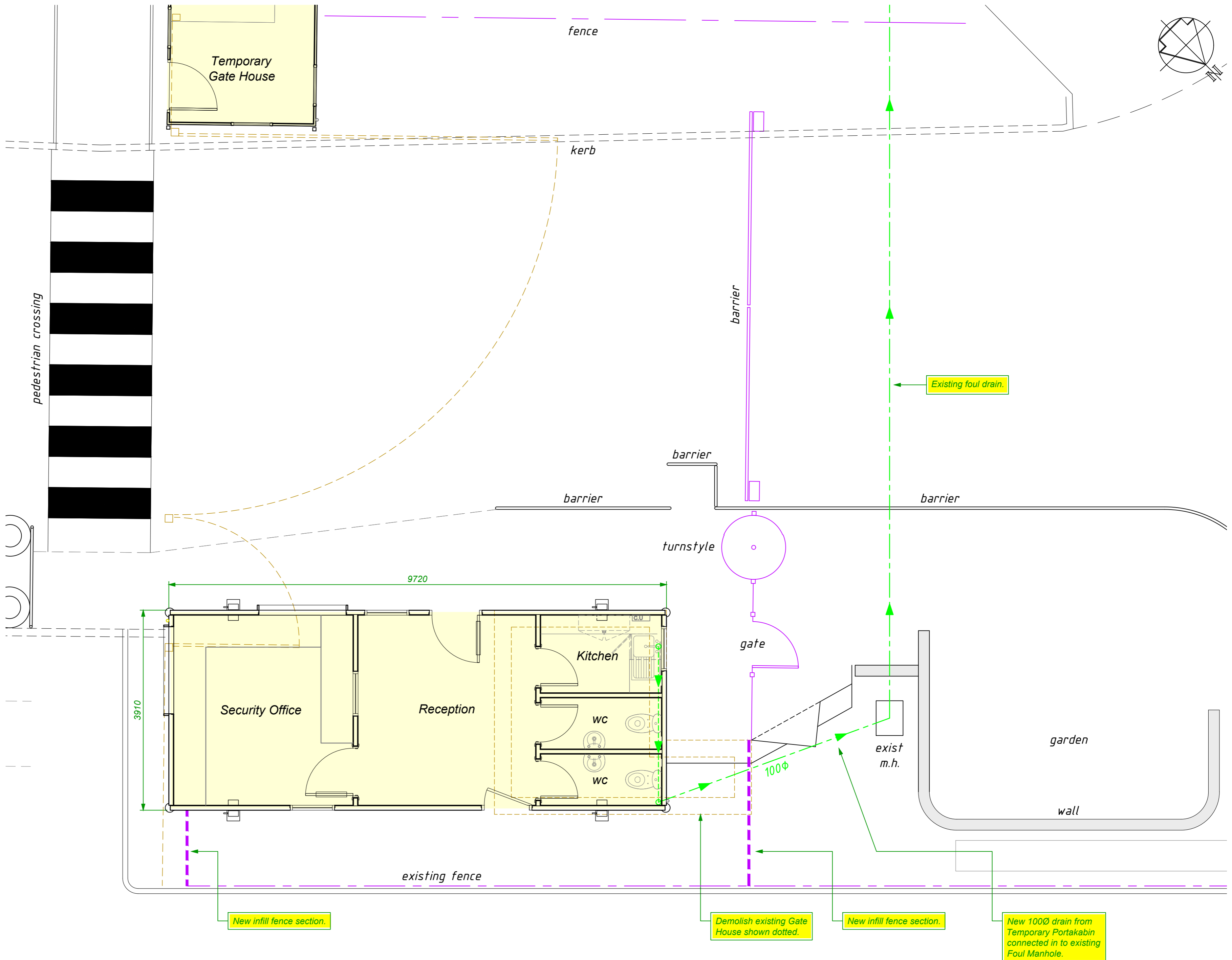
PLAN- scale 1:50
