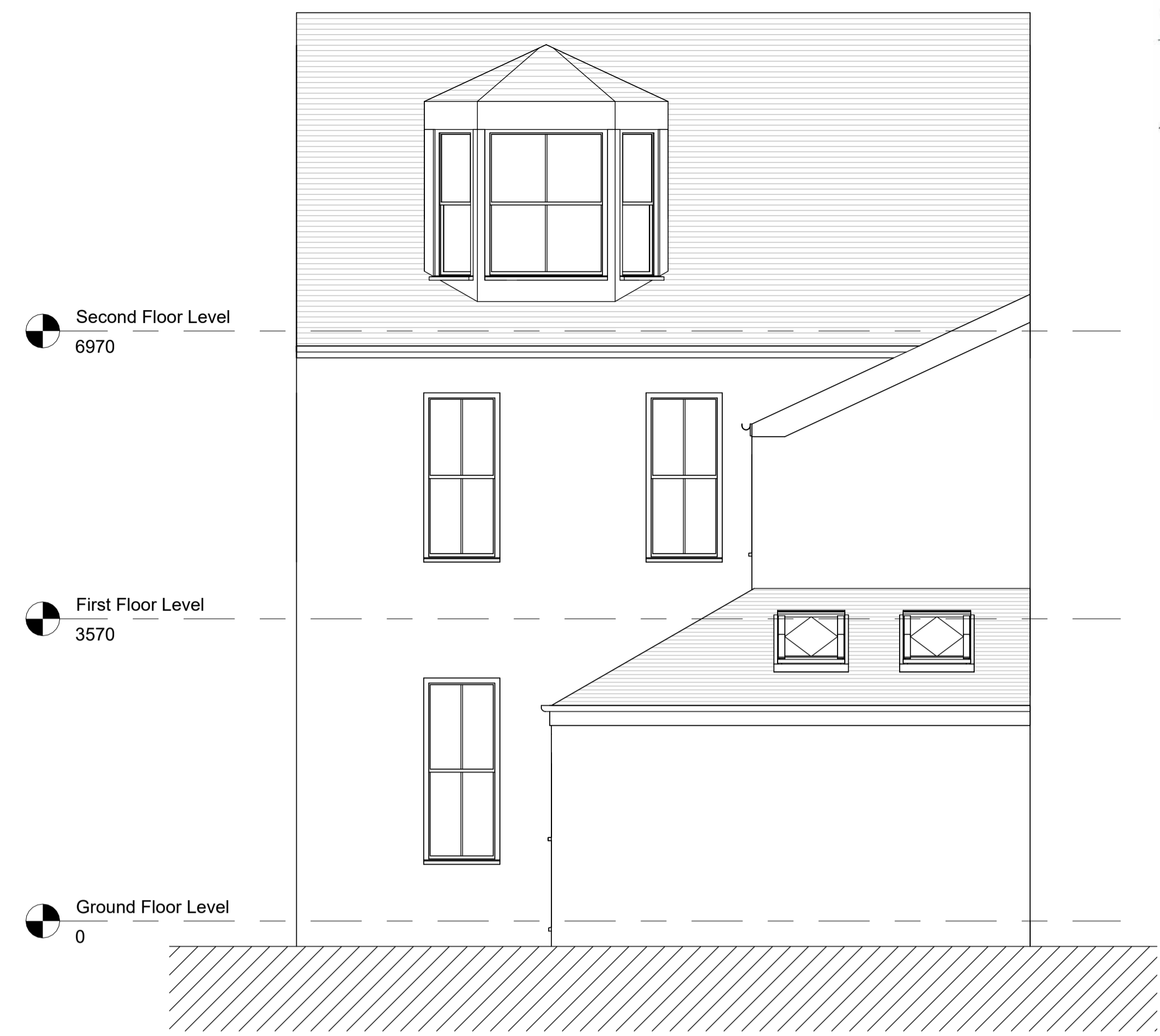
2 Existing South Elevation 1 : 50
