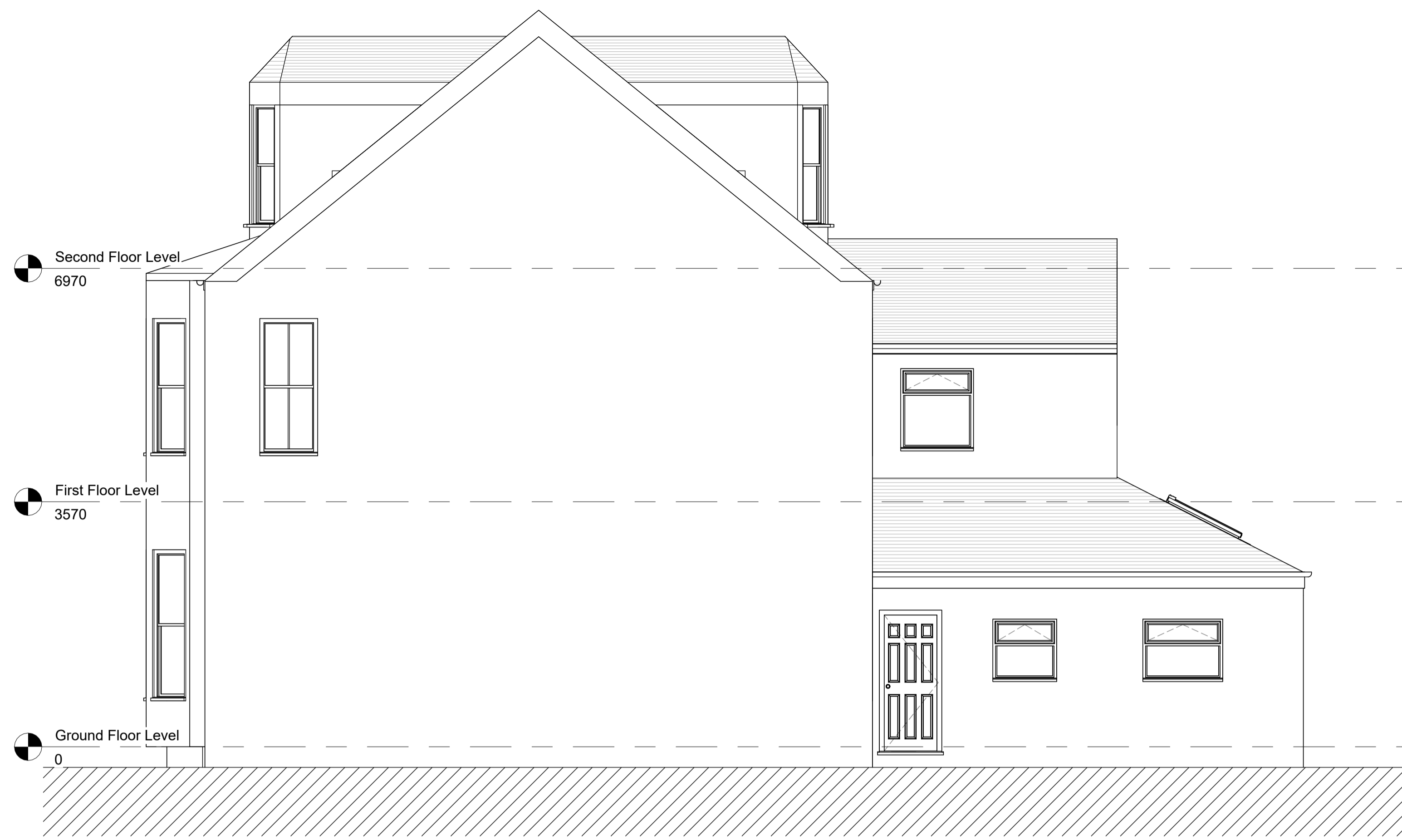
1 Existing West Elevation 1 : 50
