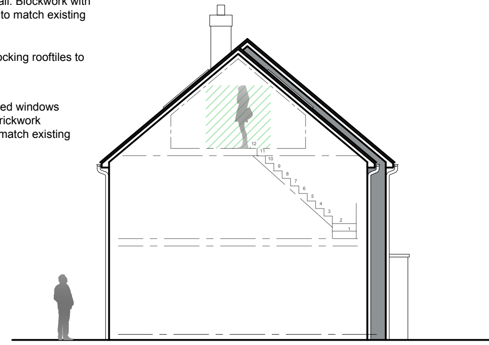
Side (south)
