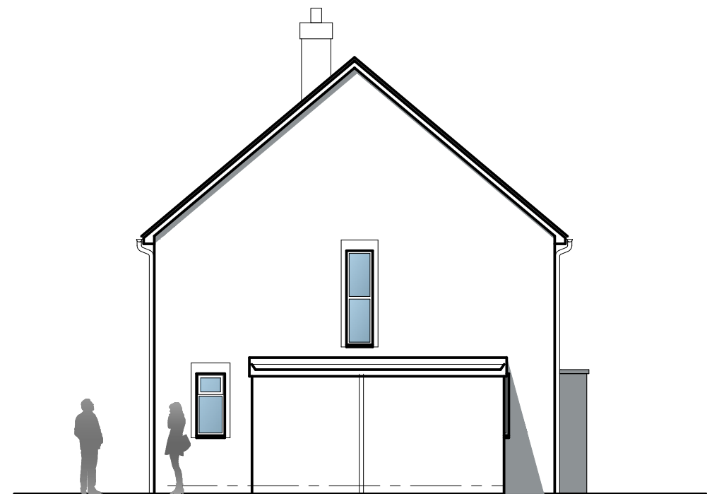
Side (south)
