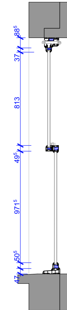
Proposed Section 1:20
