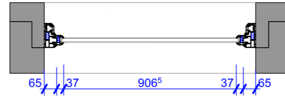
Proposed Plan 1:20
