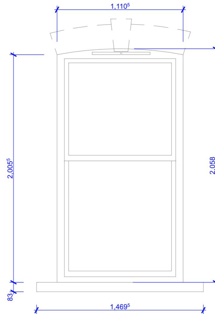
Proposed Elevation 1:20
