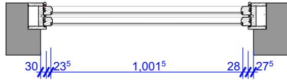
Existing Plan 1:20
