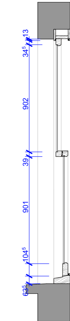
Existing Section 1:20
