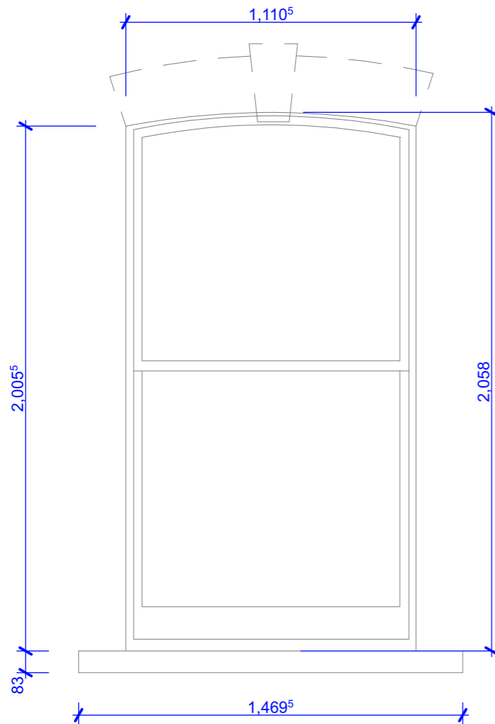
Existing Elevation 1:20
