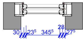
Existing Plan 1:20
