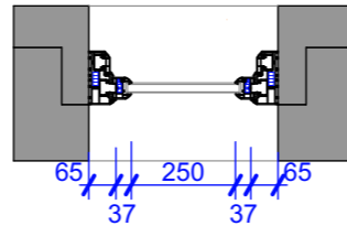
Proposed Plan 1:20
