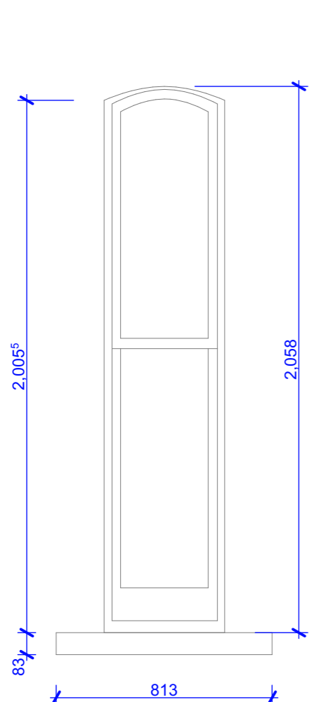
Existing Elevation 1:20
