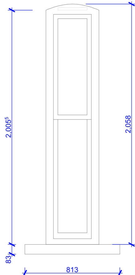
Proposed Elevation 1:20
