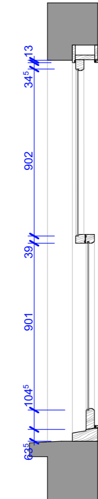
Existing Section 1:20
