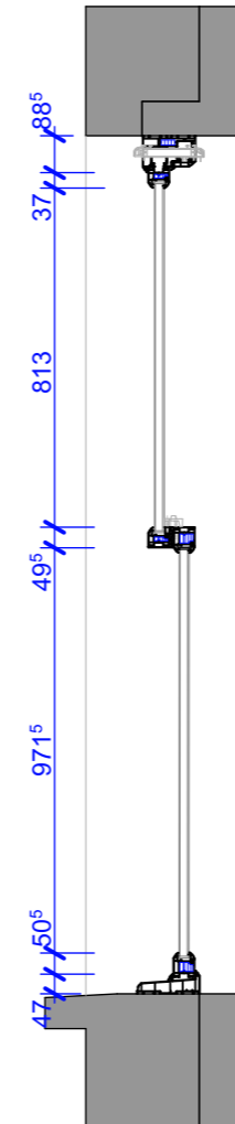
Proposed Section 1:20
