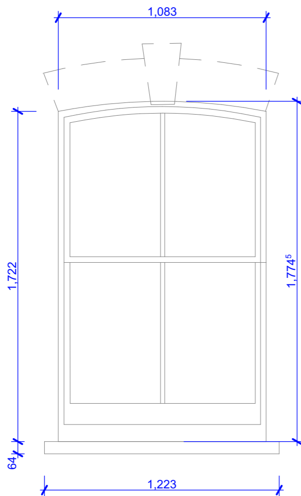
Existing Elevation 1:20
