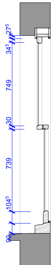
Existing Section 1:20
