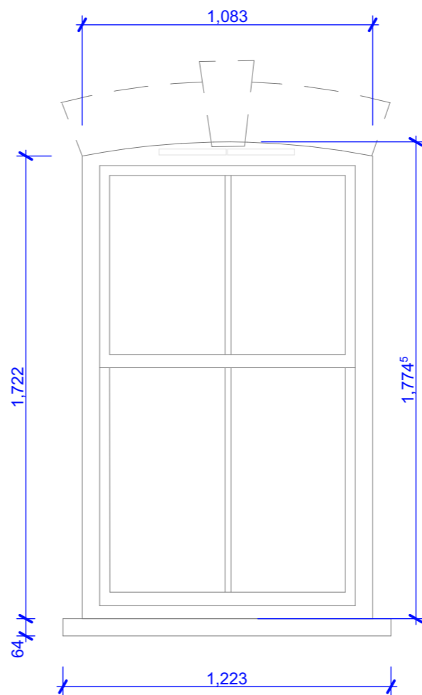
Proposed Elevation 1:20
