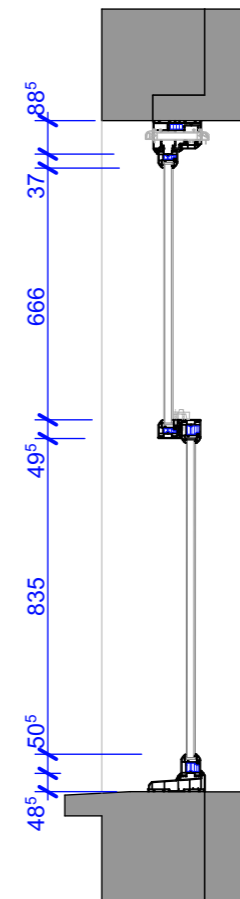
Proposed Section 1:20
