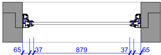
Proposed Plan 1:20
