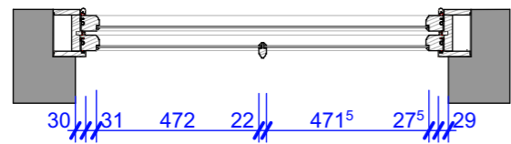
Existing Plan 1:20
