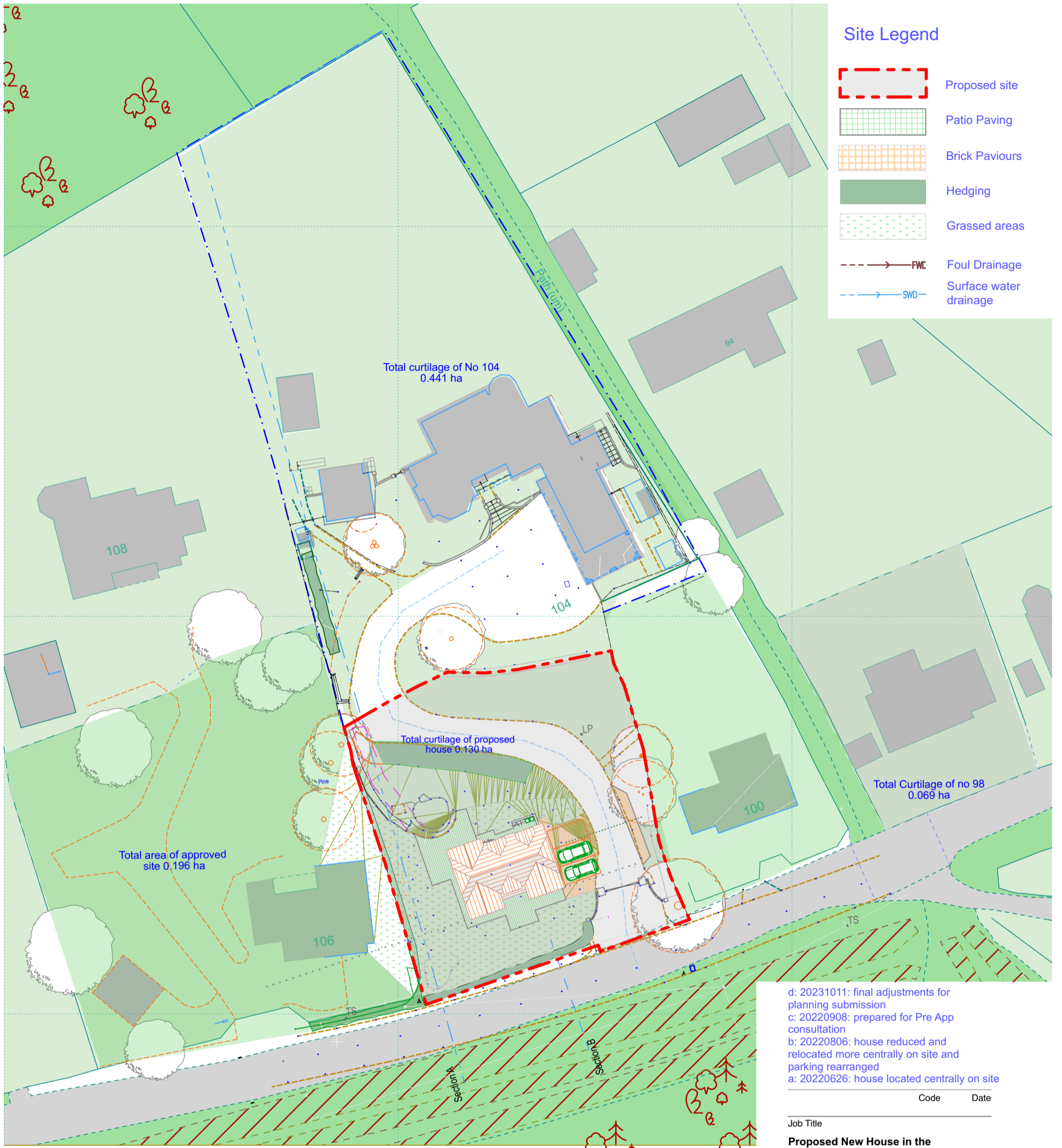
0. Block Plan 1:500
