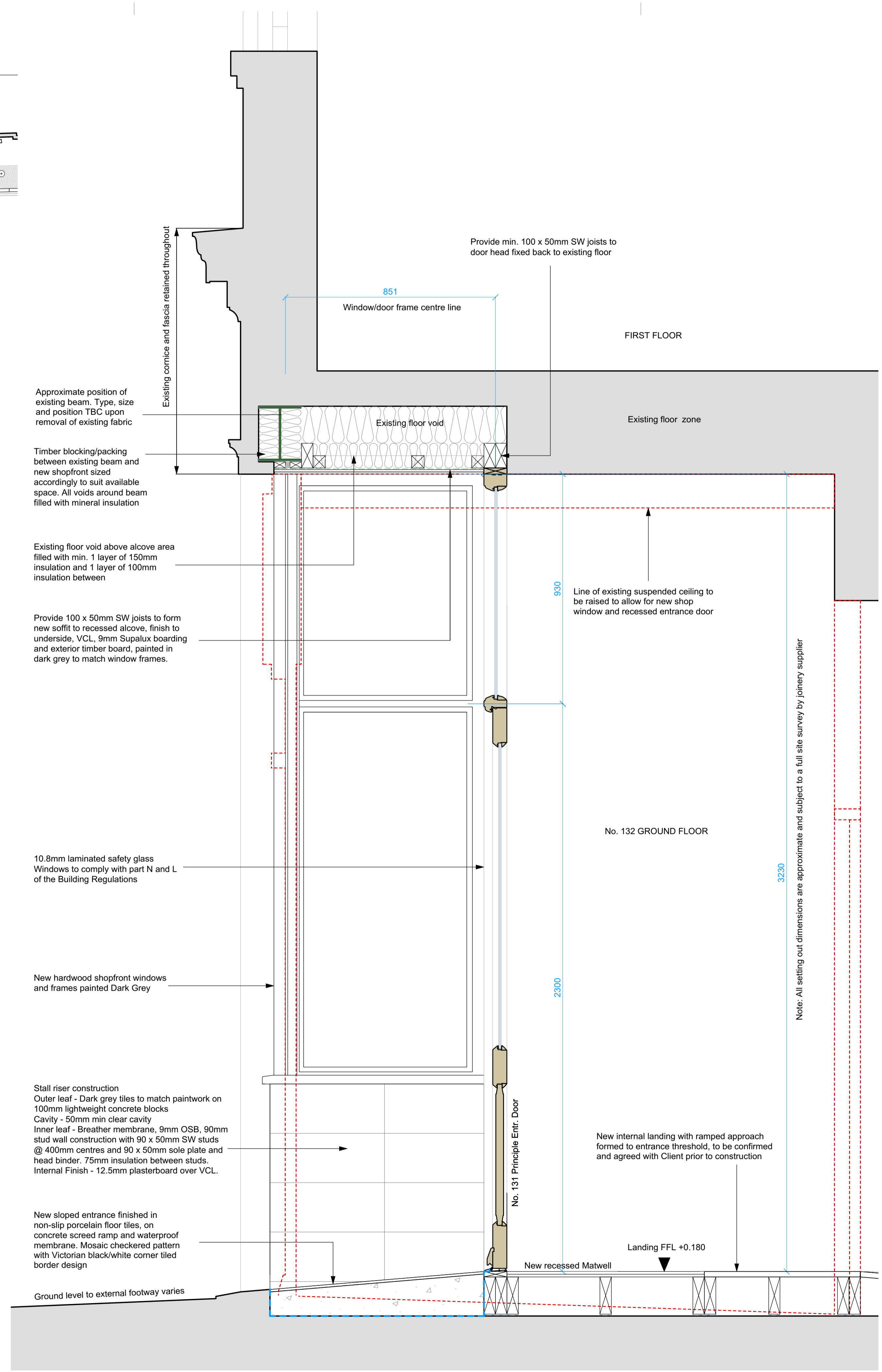
SECTION C-C
