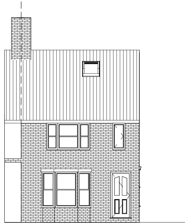
1 Existing Front Elevation 1 : 100
