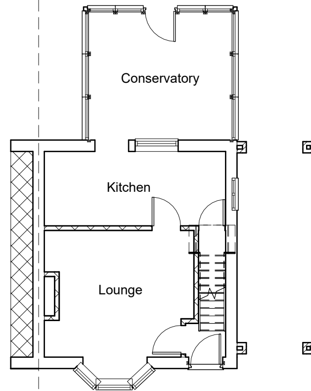
2 Proposed Ground Floor 1 : 100
