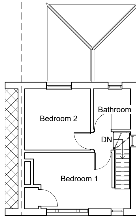
3 Existing First Floor 1 : 100
