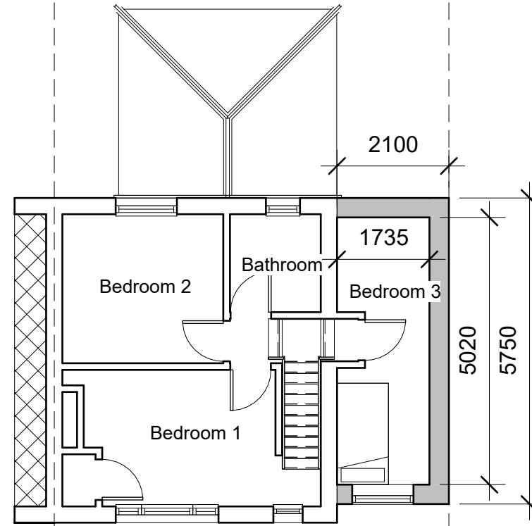
4 Proposed First Floor 1 : 100
