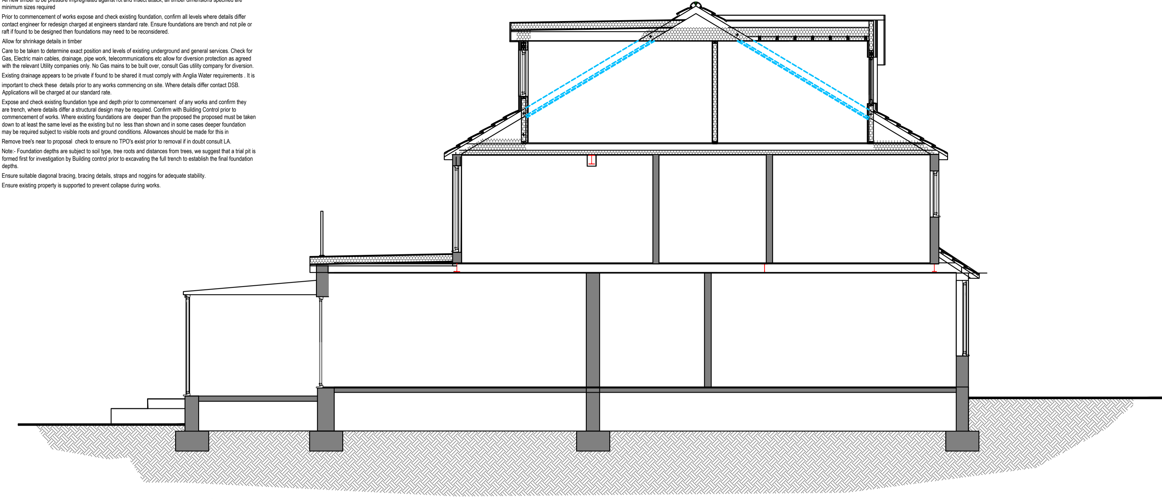
24 Proposed Section A-A 1:50 All dimensions and measurements contained on this drawing are approximate and it is the responsibility of the Contractor to ascertain all accurate dimensions and measurements on site.
