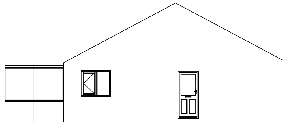
9725 Side (South) Elevation
