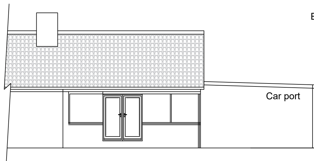
Rear Elevation
