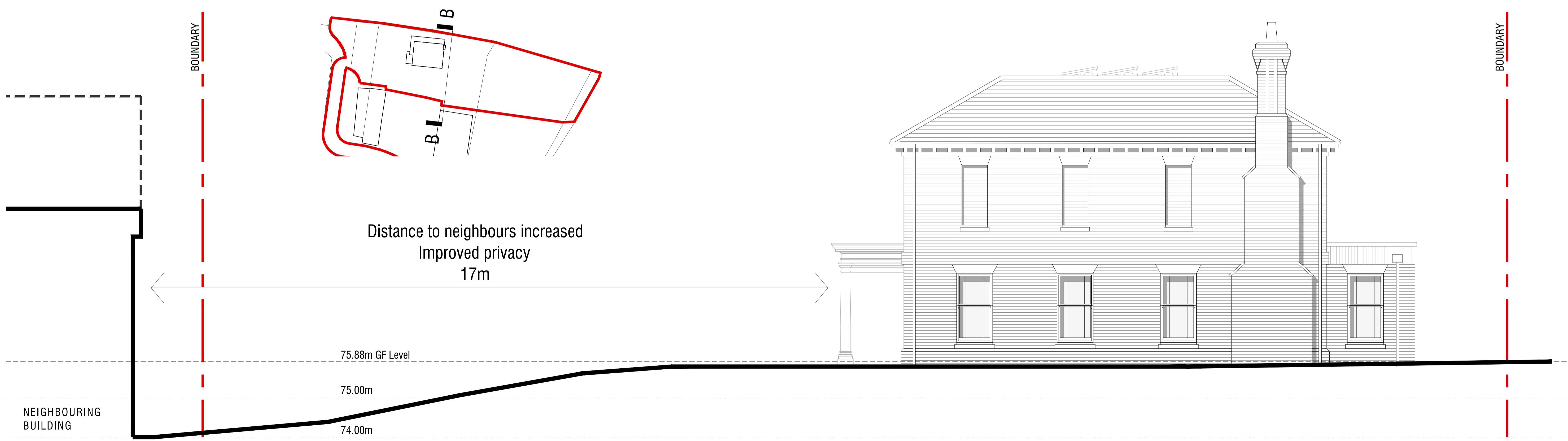
SITE SECTION BB proposed | east 1:50
