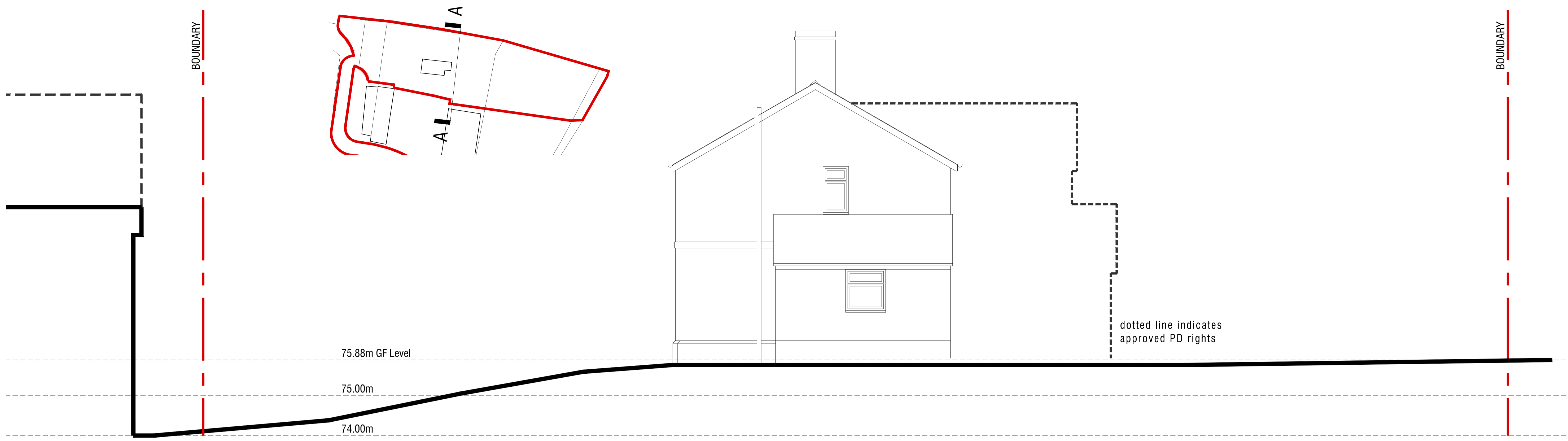
SITE SECTION AA existing | east 1:50
