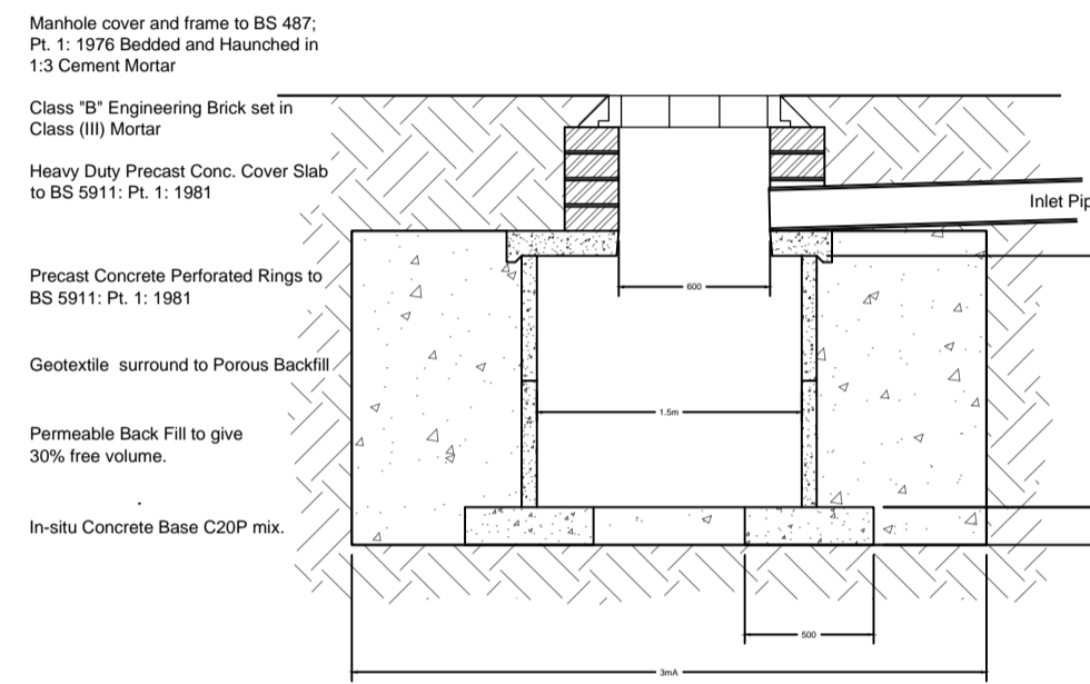
Typical Soakaway Detail (allow for 5 No.)
