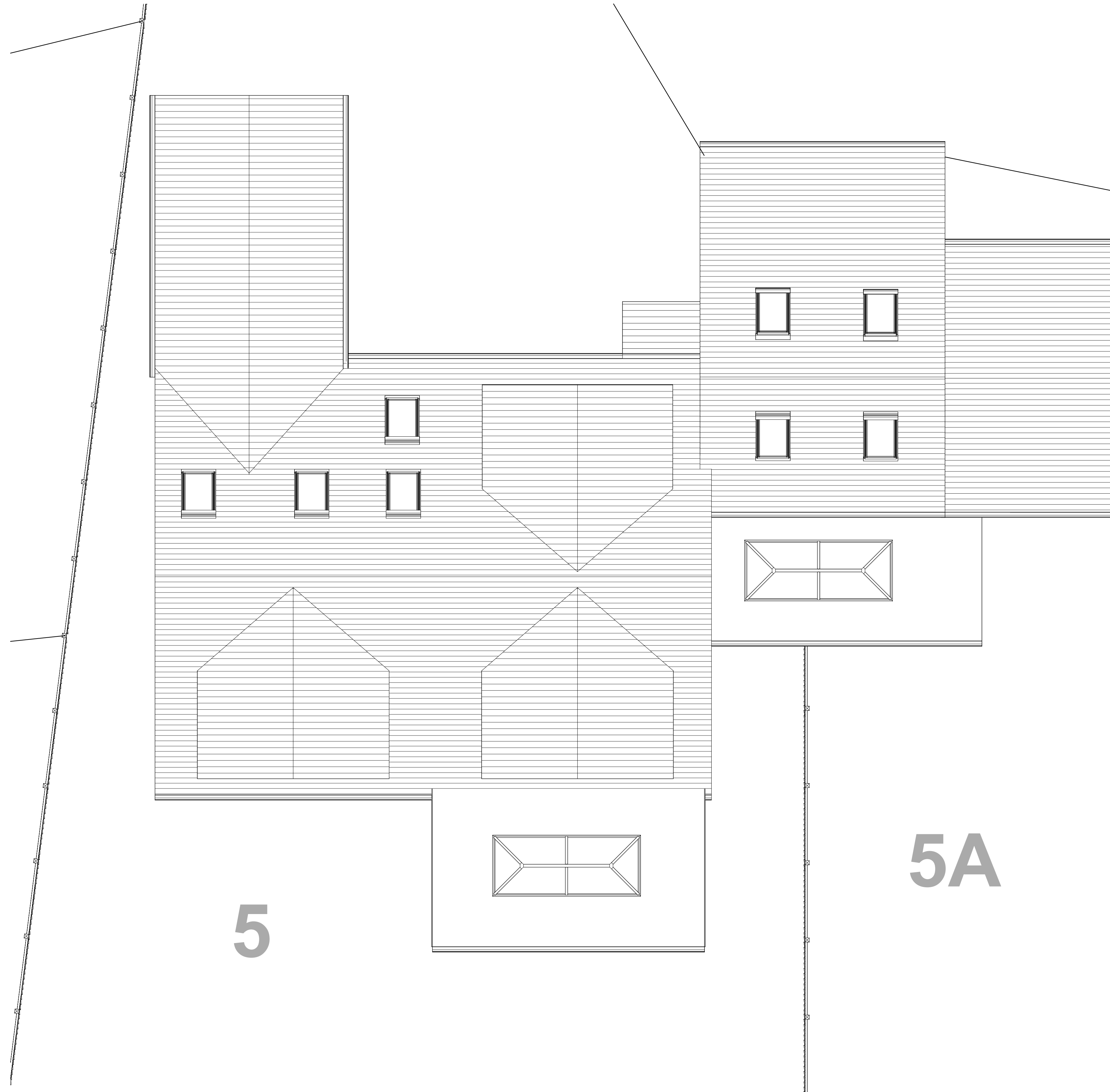
Site_Proposed 1 : 50
